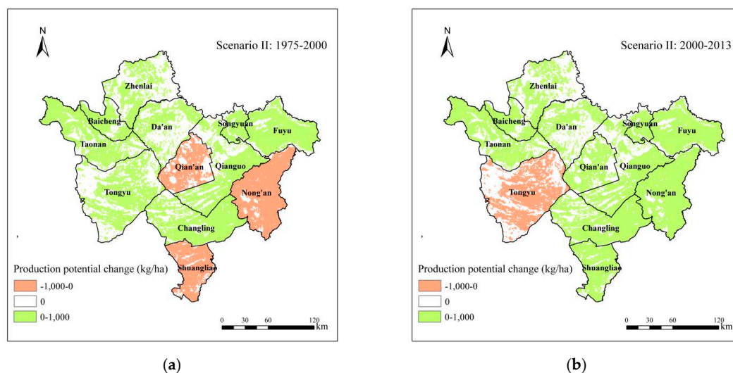
Figure 10. Spatial distribution of soybean production potential change between 1975 and 2000, and between 2000 and 2013 under Scenario II. (a) between 1975 and 2000; (b) between 2000 and 2013.
