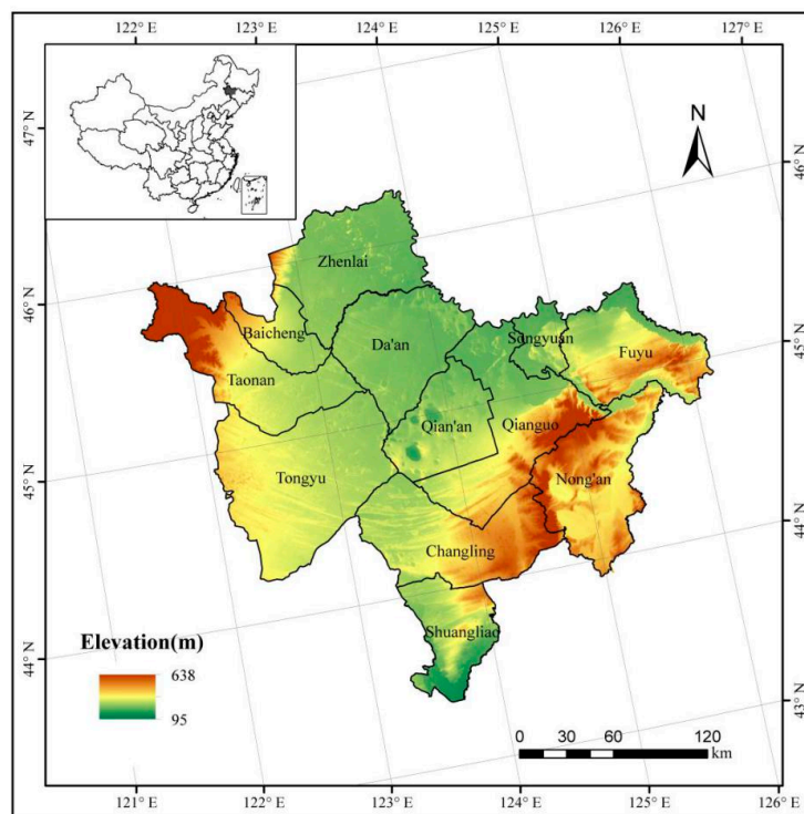
Figure 1. Location of Western Jilin, China.
